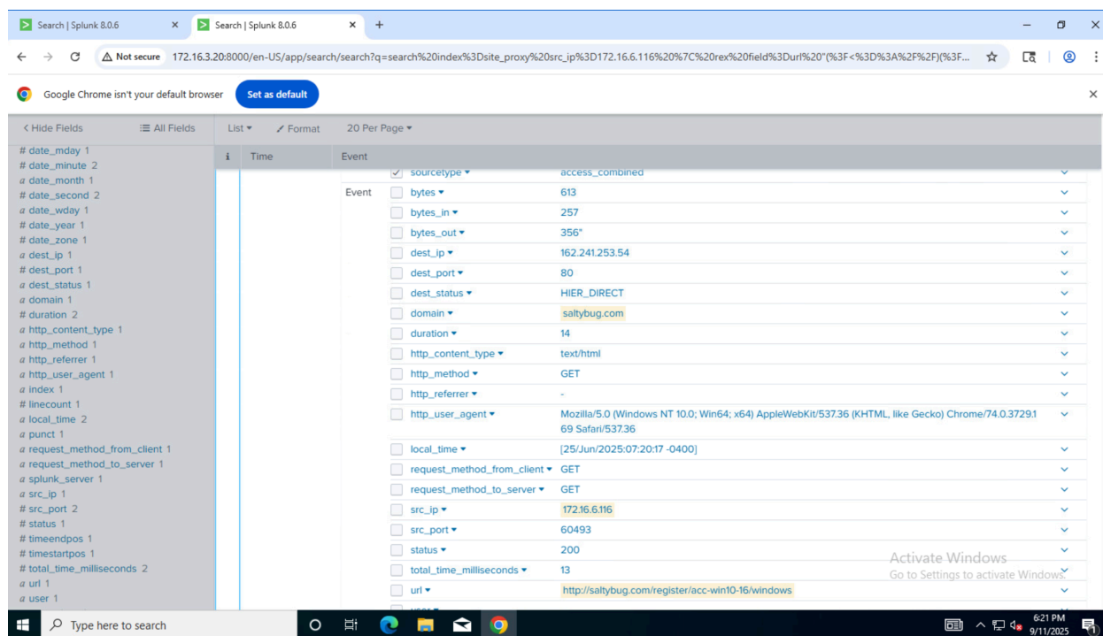
Figure 1: acc-win10-16 being registered with saltybug
