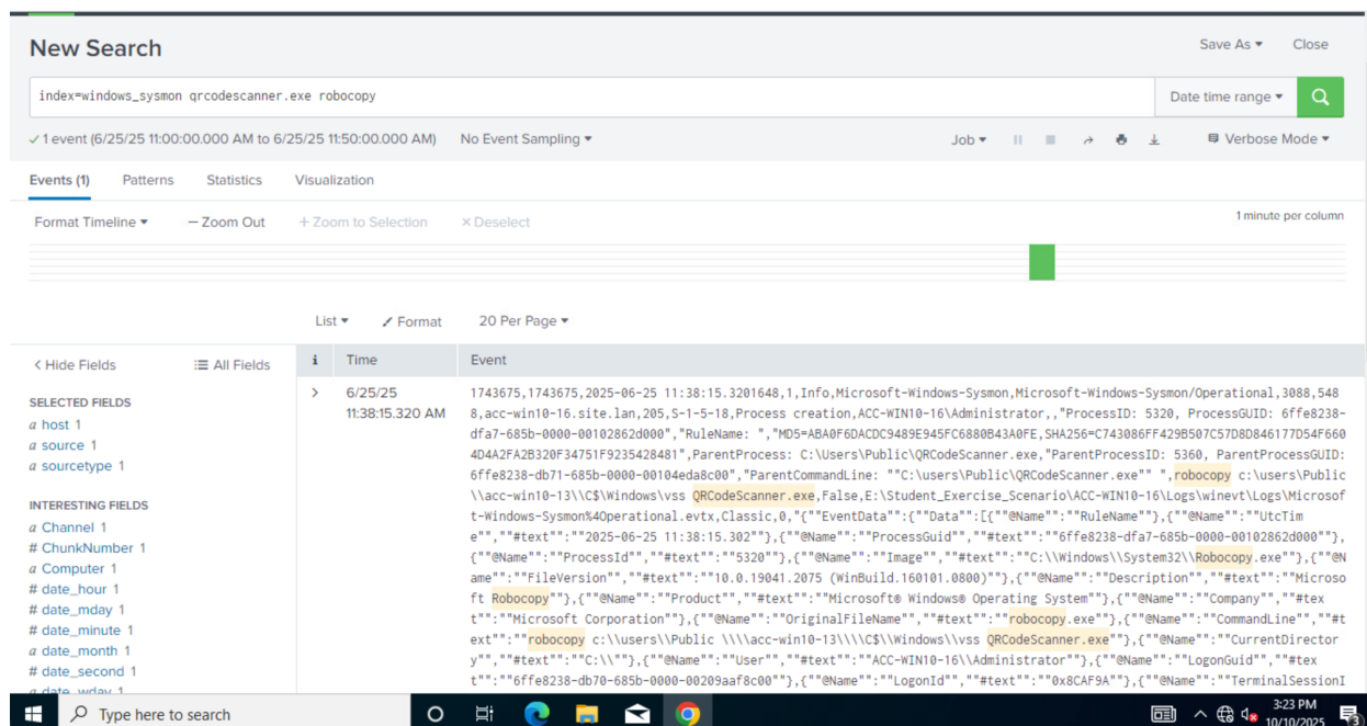
Figure 2: Attacker copying QRCodeScanner.exe to acc-win10-13
